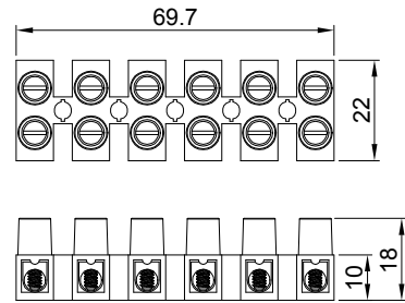
Screw Terminal Blocks
