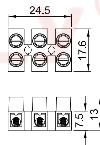
Screw Terminal Blocks
