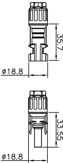
1000VDC PV4.0 Diode Connector
