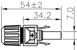
Female connector
