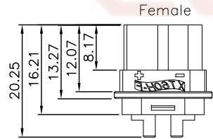
DS1171-03 SERIES Scale:2:1
