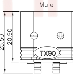
DS1171-04 SERIES Scale:2:1
