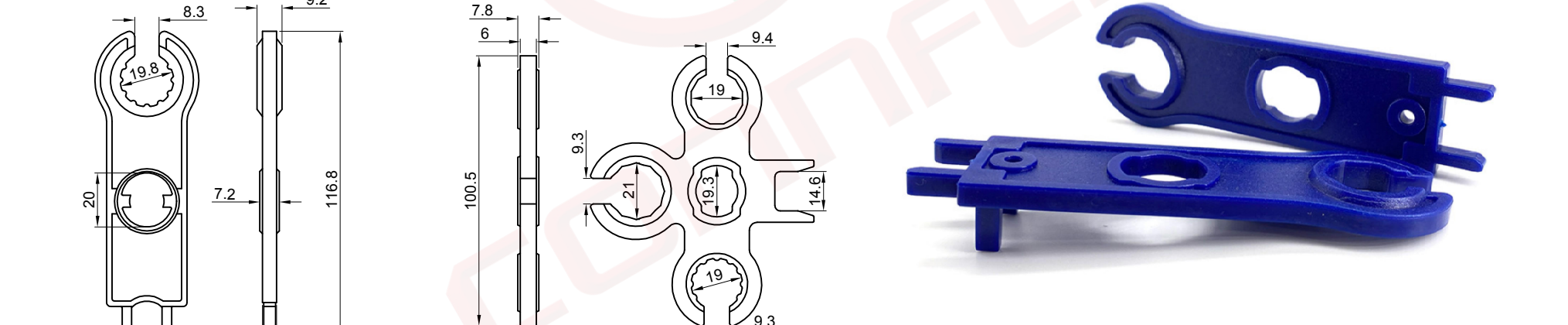
Type 3(1500V Round type) Type 4(Multifunction type)
