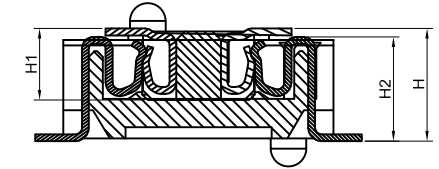
Mating height With DS1151-04
