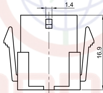
8Pin Male housing
