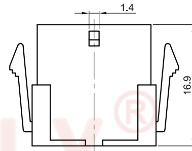
10Pin Male housing
