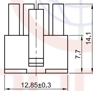
8Pin Female housing
