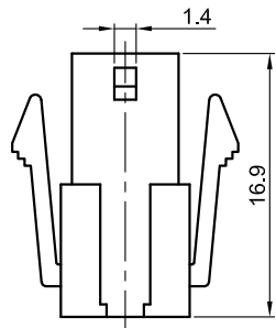
4Pin Male housing
