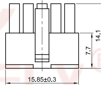
10Pin Female housing
