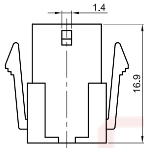
6Pin Male housing
