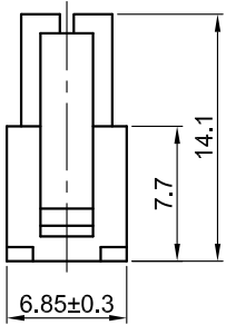
4Pin Female housing
