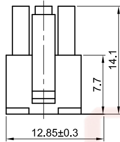
6Pin Female housing
