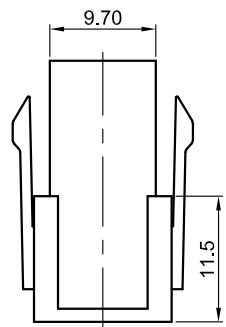
2Pin Male V/T Type
