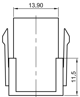
3Pin Male V/T Type
