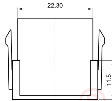
5Pin Male V/T Type
