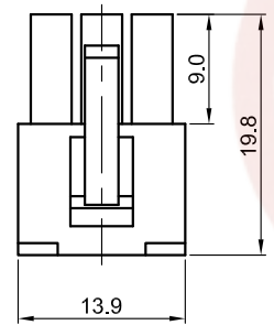
3Pin Female housing
