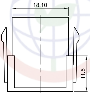
4Pin Male V/T Type
