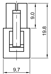
2Pin Female housing
