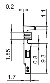
Female contact
