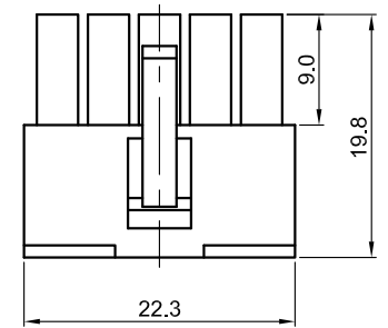
5Pin Female housing
