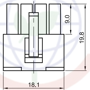
4Pin Female housing
