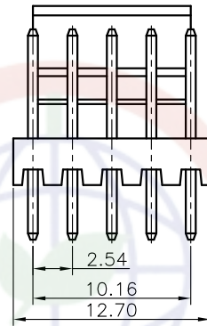
5Pin Male V/T Type
