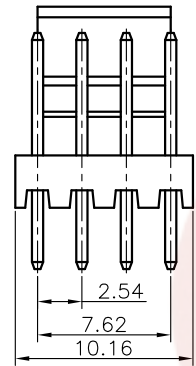
4Pin Male V/T Type
