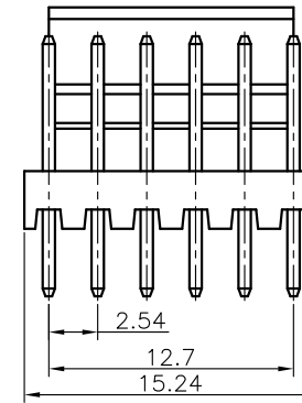
6Pin Male V/T Type
