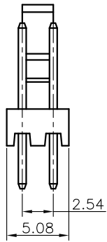
2Pin Male V/T Type
