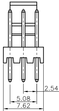
3Pin Male V/T Type
