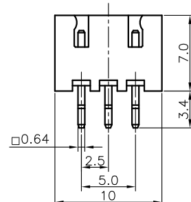
3Pin Male V/T Type
