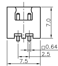
2Pin Male R/A Type
