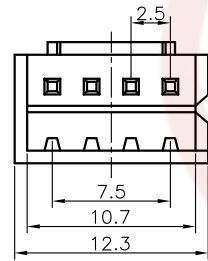
4Pin Female housing
