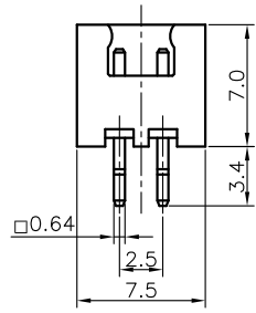
2Pin Male V/T Type
