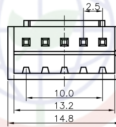
5Pin Female housing
