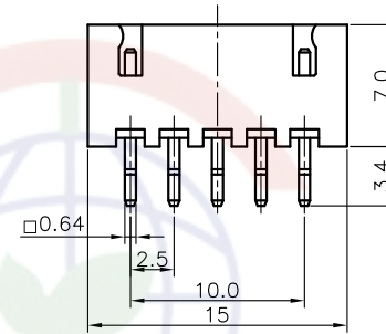
5Pin Male V/T Type
