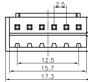
6Pin Female housing
