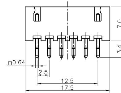
6Pin Male V/T Type
