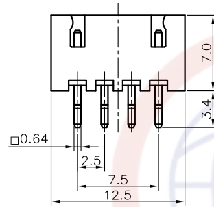
4Pin Male V/T Type
