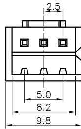
3Pin Female housing
