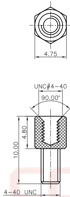
4.8x10mm 4-40UNC Screw
