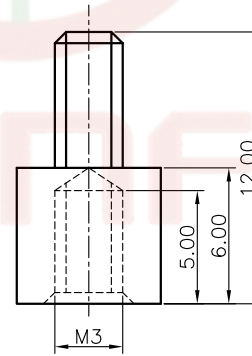
5.5x12mm M3 Screw
