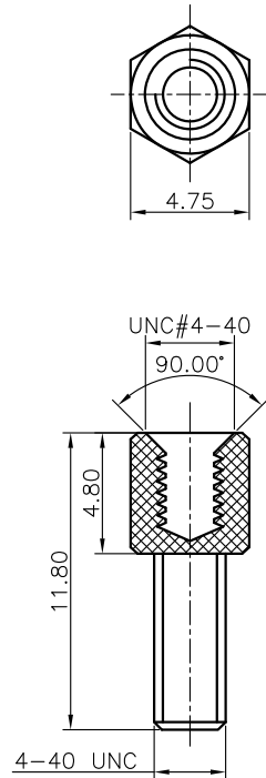
4.8x11.8mm 4-40UNC Screw
