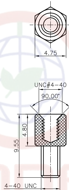
4.8x9.55mm 4-40UNC Screw
