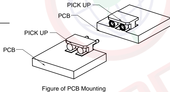
Figure of PCB Mounting
